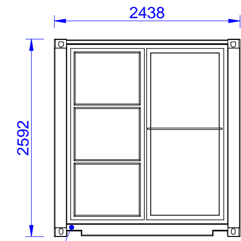
FRONT END VIEW 1:50
